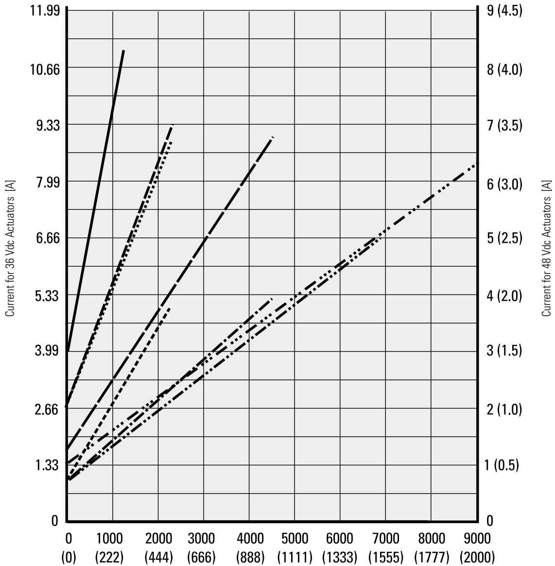
Load vs. Current for 36 and 48 Vdc actuators
